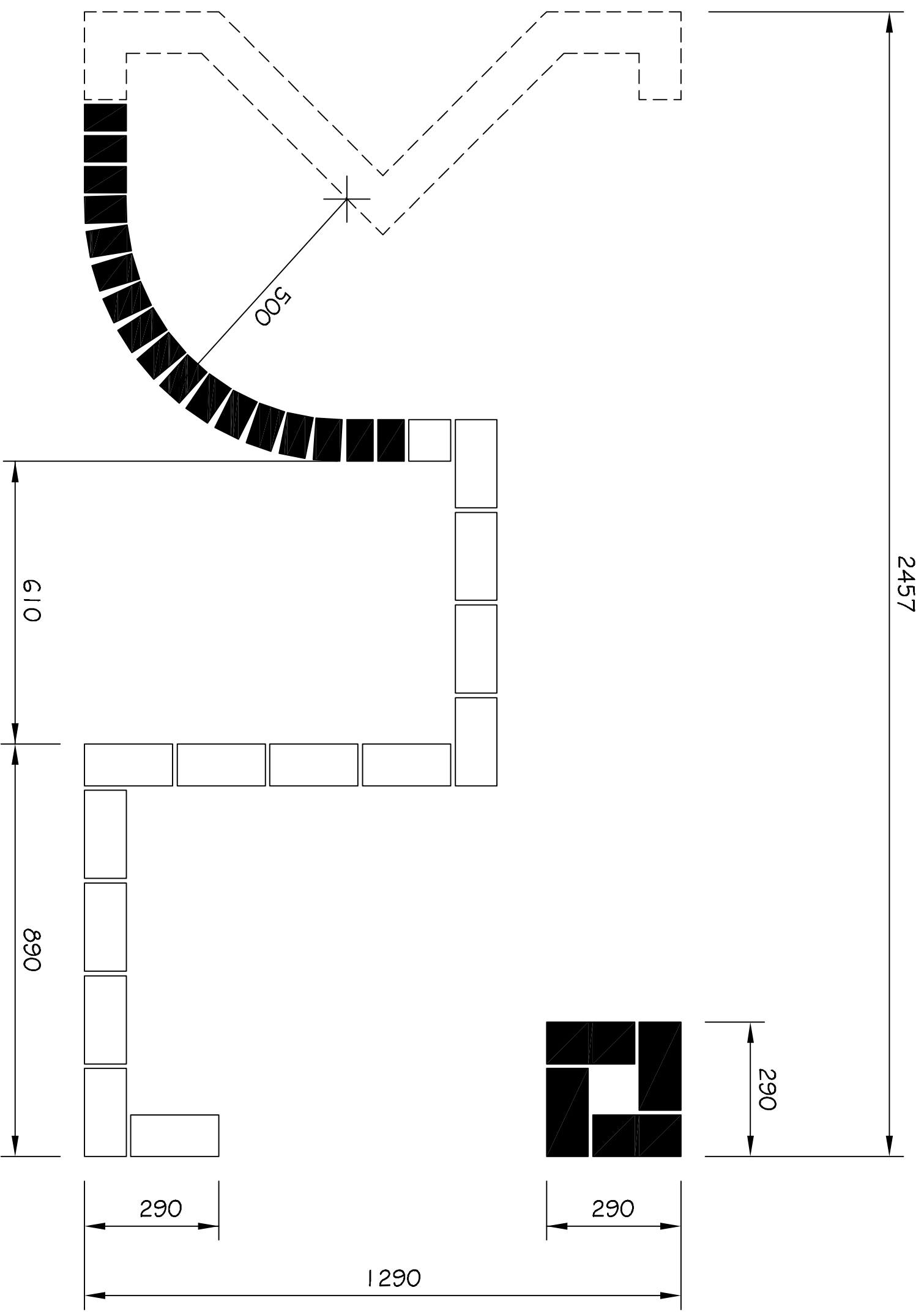
PLAN - (Course 1)
