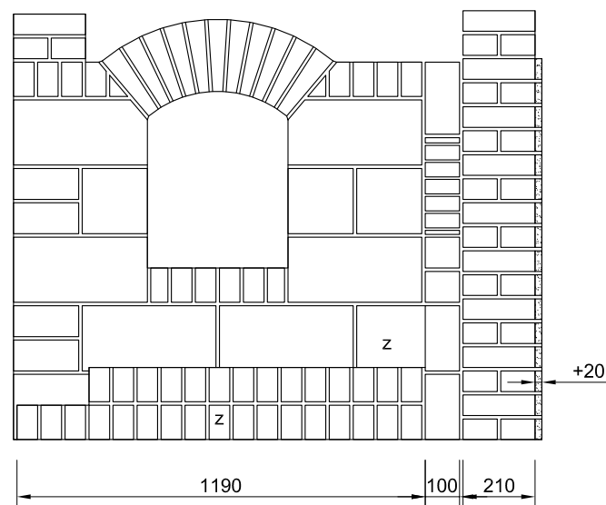
VIEW A
