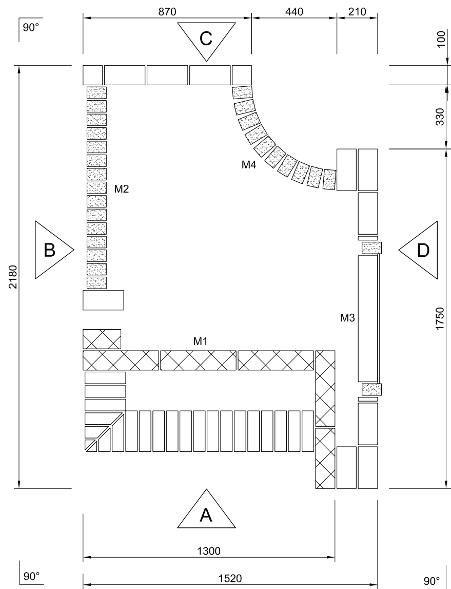
PLAN-COURSE 1
