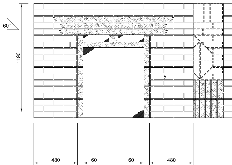
VIEW D
