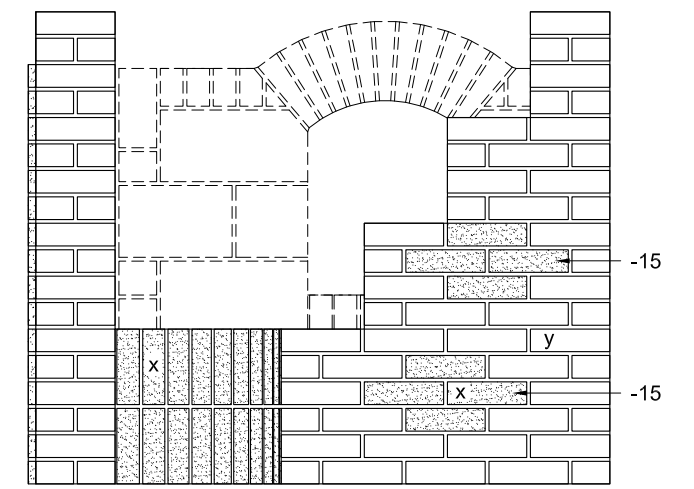
VIEW C
